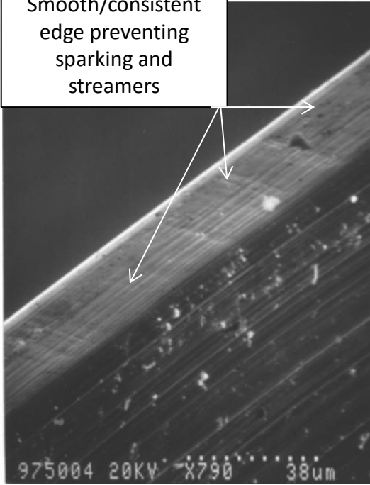
(SEM Image of Avocet Precision Pinning Band)
